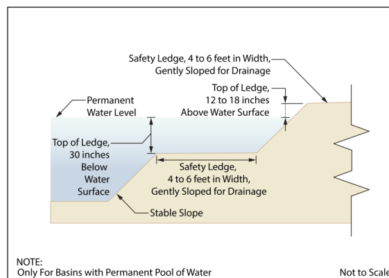
Elevation View — Basin Safety Ledge Configuration
